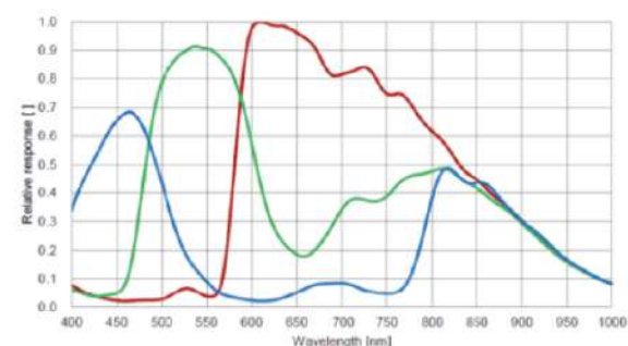
MV-CS004-10UC
